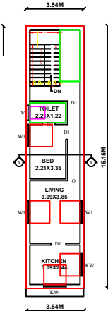
PROPOSED SECOND FLOOR PLAN (RESIDENTIAL)
