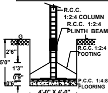
FOUNDATION DETAIL
