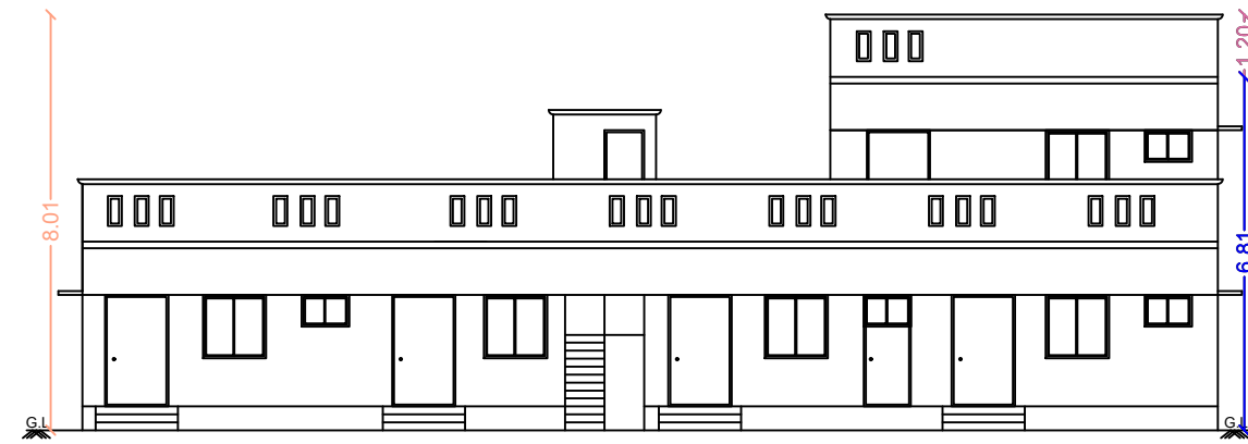
FRONT ELEVATION
