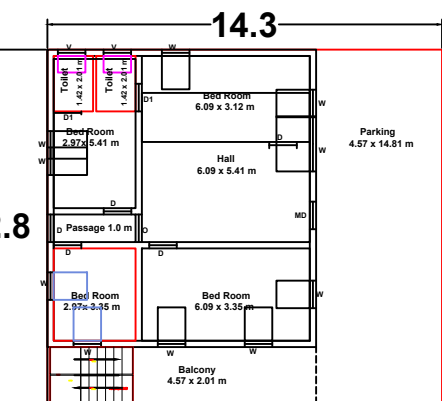
EXISTING GROUND FLOOR (BLOCK-1)
