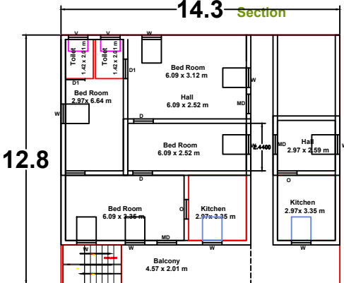
EXISTING FIRST FLOOR (BLOCK-1)
