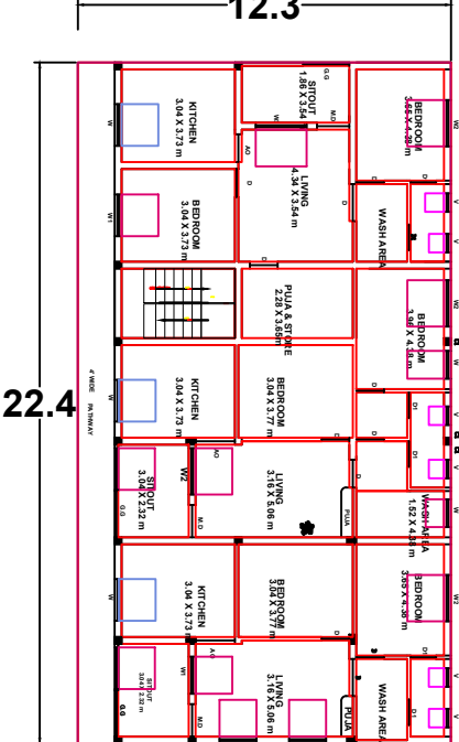
PROPOSED GROUND FLOOR (BLOCK-2)
