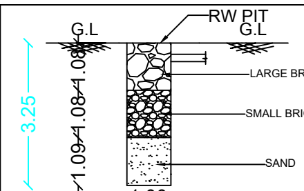
SECTION OF RAIN WATER HARVESTING PIT
