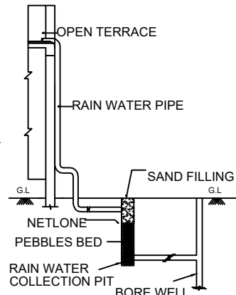
RAIN WATER
