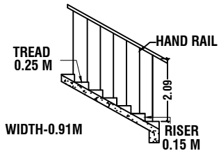
STAIRCASE DETAILS
