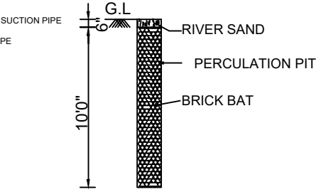
PERCOLATION PIT
