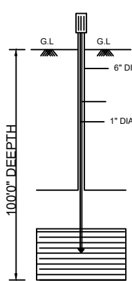
BORE WELL
