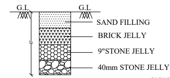
RAIN WATER HARVESTING RECHARGE PIT
