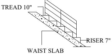
STAIRCASE DETAILS [N.T.S.]
