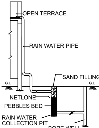
RAIN WATER
