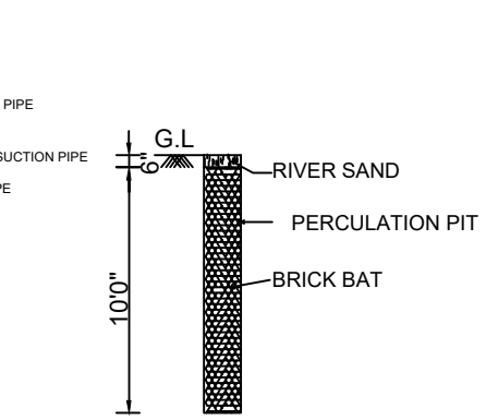
PERCUSSION PIT
