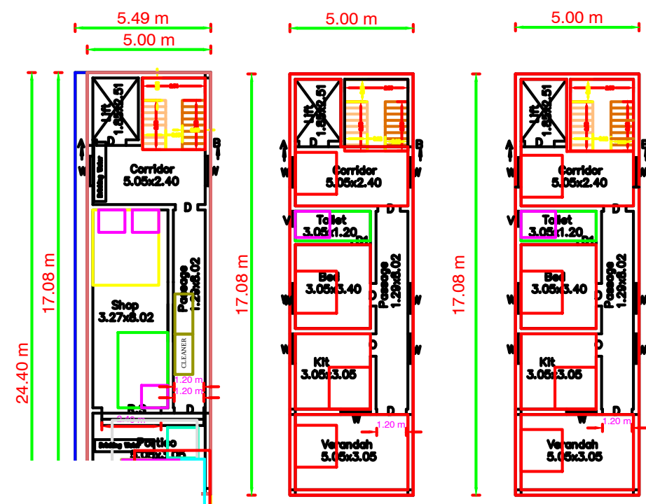
Pro.First Floor Pro.Second Floor
