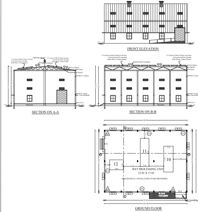
BLOCK 3 - WET PROCESSING UNIT
