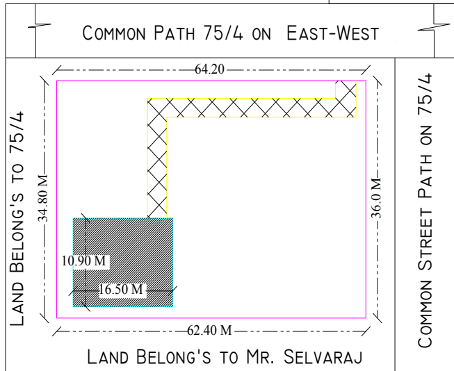
KEY PLAN (As Per Site Location)
