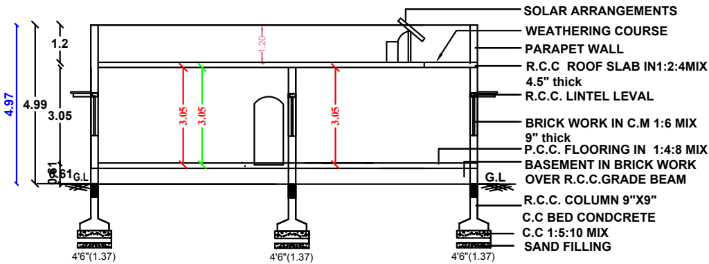
SECTION " AB "
