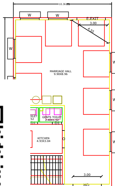
NG GROUND FLOOR PLAN Already approved) Permission No: 05/2024-2025/NGI
