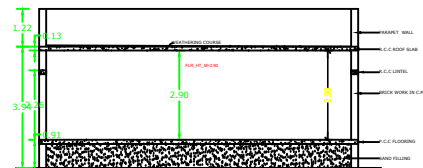
SECTION ON K-S
