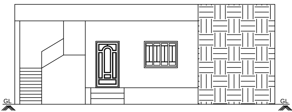
FRONT ELEVATION (NORTH FACING)
