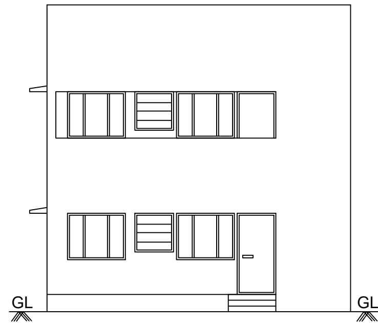
FRONT ELEVATION
