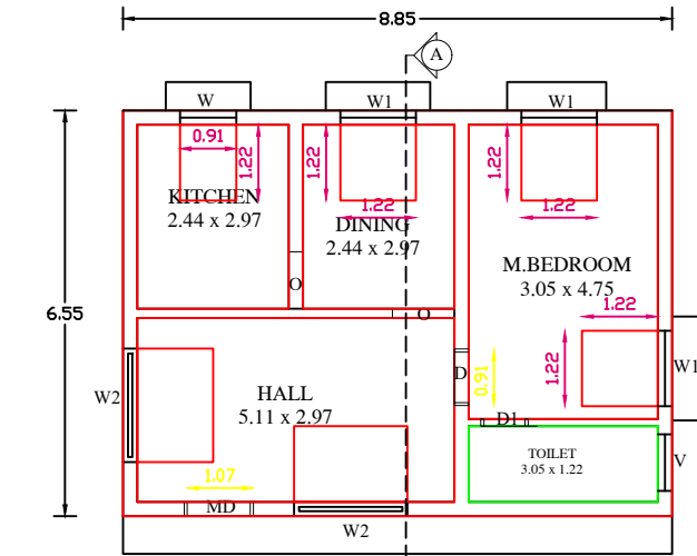
PROPOSED GROUND FLOOR PLAN (FACING NORTH)
