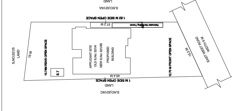
SITE PLAN (SCALE 1: 2)
