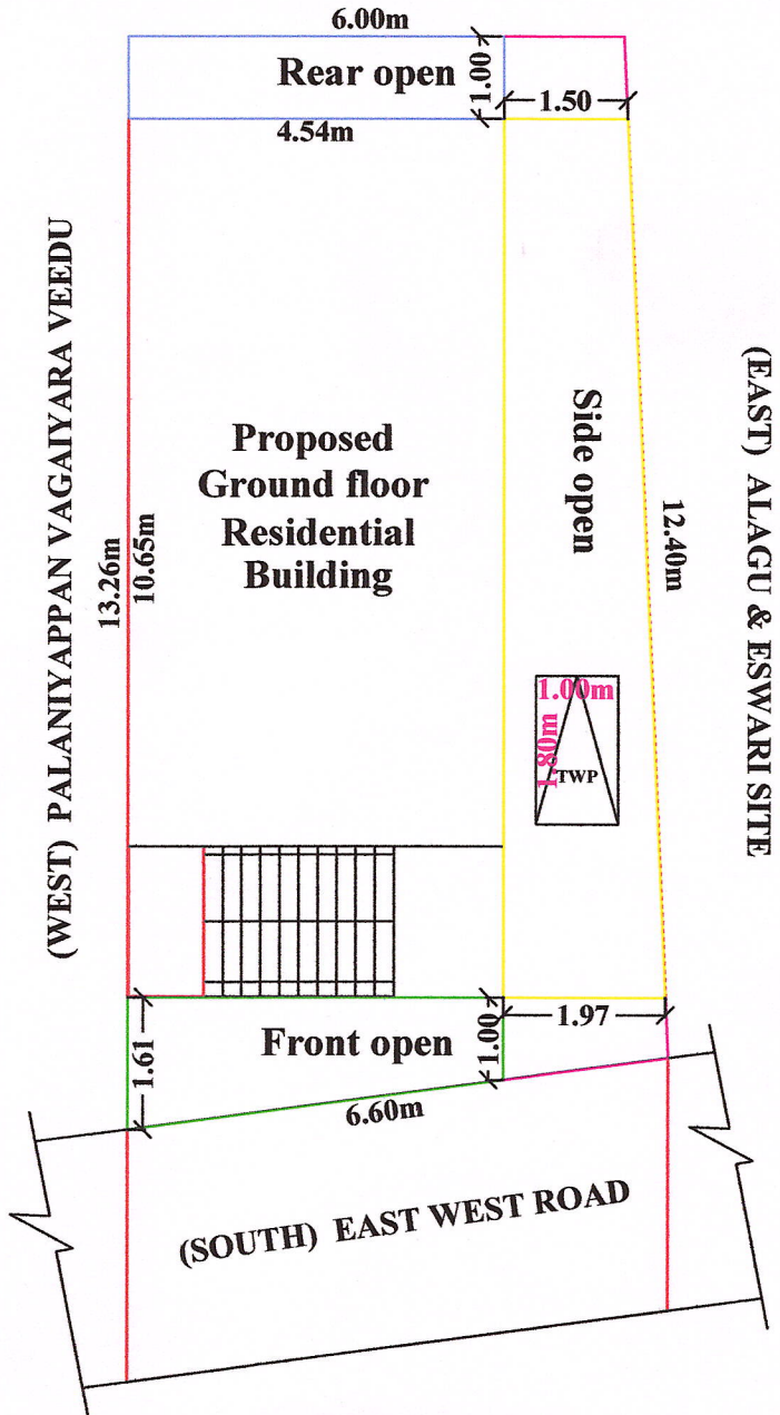
SITE PLAN
