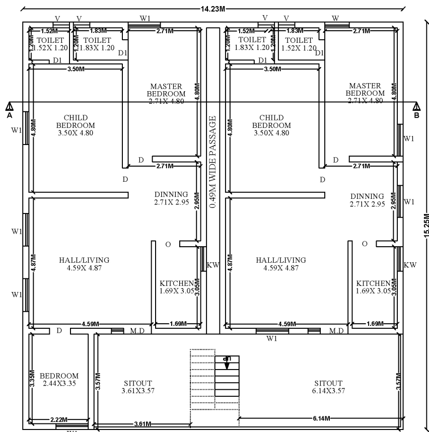
PROPOSED FIRST FLOOR & SECOND FLOOR PLAN
