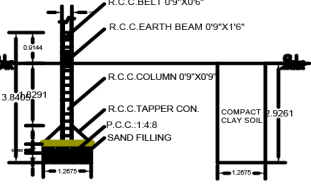
FOUNDATION DETAILS-MIDDLE COLUMN
