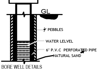
BORE WELL DETAILS
