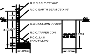
FOUNDATION DETAILS-END COLUMN
