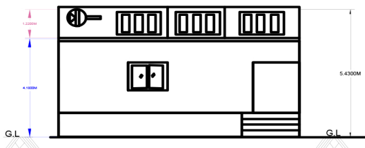
FRONT ELEVATION
