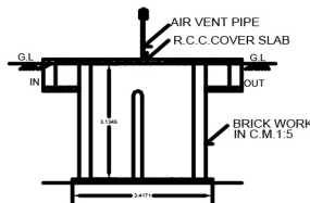
SEPTIC TANK DETAILS-SECTION
