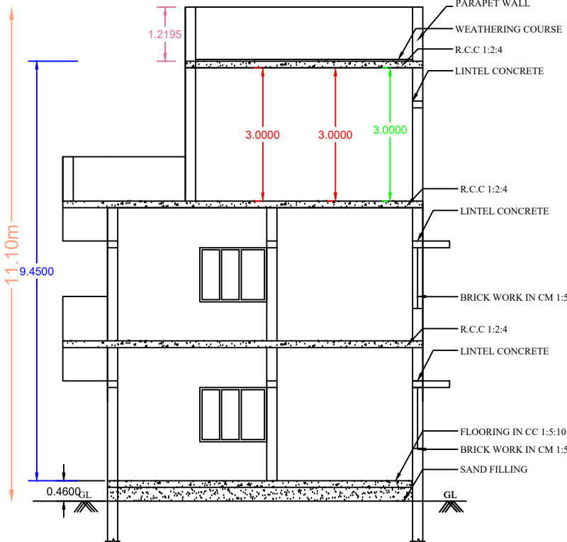
SECTION AB
