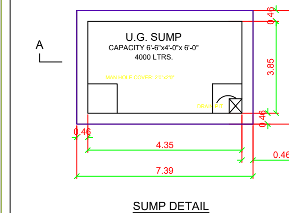
SUMP DETAIL
