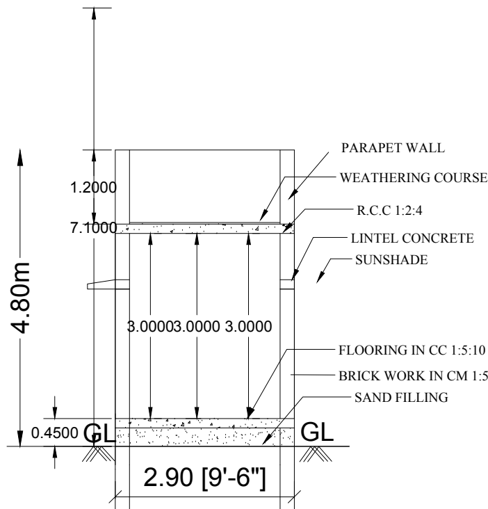
SECTION ON AA 8.00 [26'-3"]
