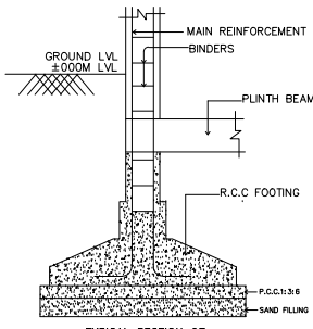
TYPICAL SECTION OF R.C.C. COLUMN FOUNDATION SCALE 1"=2'-0"
