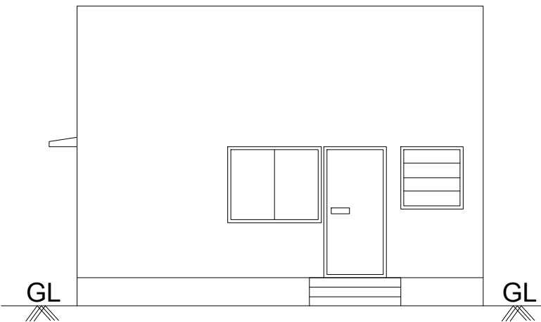
FRONT ELEVATION
