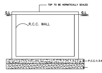
SECTION ON AA U.G. SUMP CAPACITY 6'-0"X4'-0"X6'-0" 4000 LITRES SCALE 1"=4'-0"
