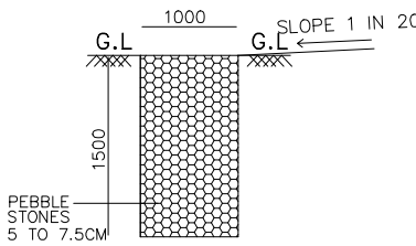
SECTION OF PEBBLE TRENCH SCALE : 1: = 100
