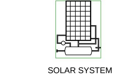
SOLAR SYSTEM
