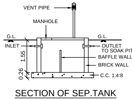
SECTION OF SEPT. TANK
