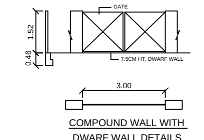
COMPOUND WALL WITH DWARF WALL DETAILS
