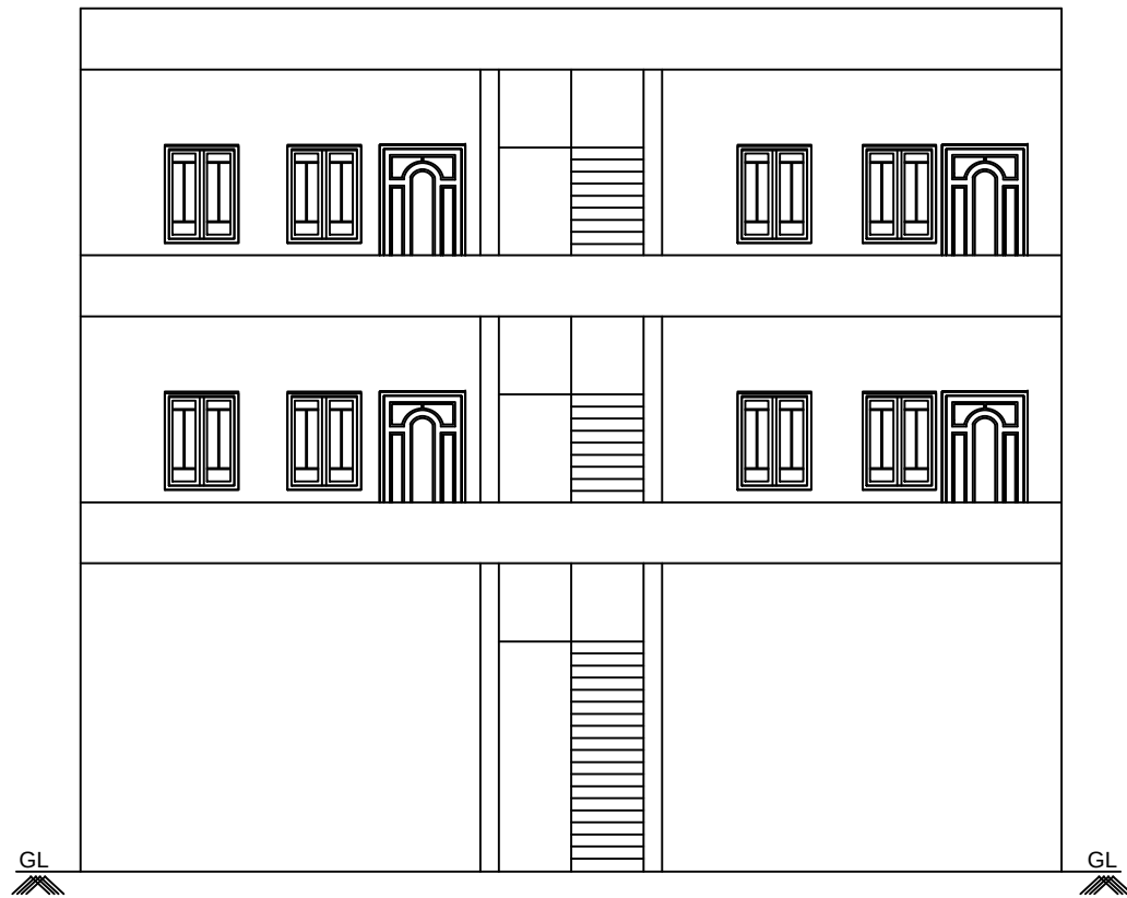
FRONT ELEVATION (EAST FACING)
