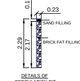
DETAILS OF SEPTIC TANK
