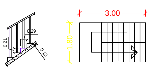
STAIRCASE DETAILS
