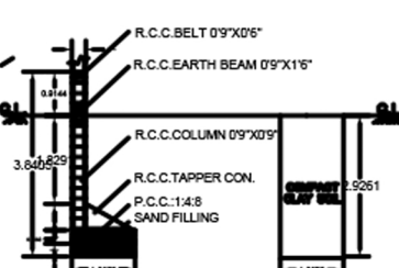
FOUNDATION DETAILS-END COLUMN
