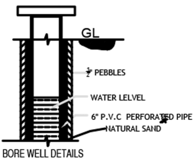
BORE WELL DETAILS
