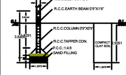
FOUNDATION DETAILS-MIDDLE COLUMN
