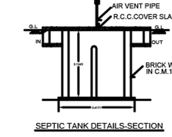
SEPTIC TANK DETAILS-SECTION
