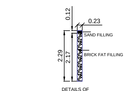
DETAILS OF PERCUSSION PIT
