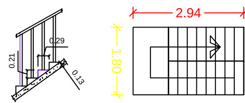
STAIRCASE DETAILS
