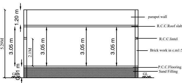
SECTION-"SR"
