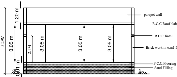
SECTION-"SR"
