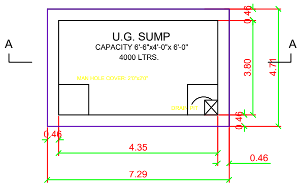
SUMP DETAIL
