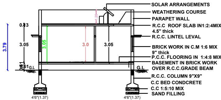
SECTION " AB "
