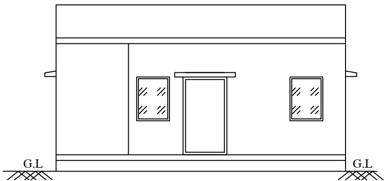
FRONT ELEVATION
