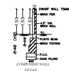
FOUNDATION DETAILS
