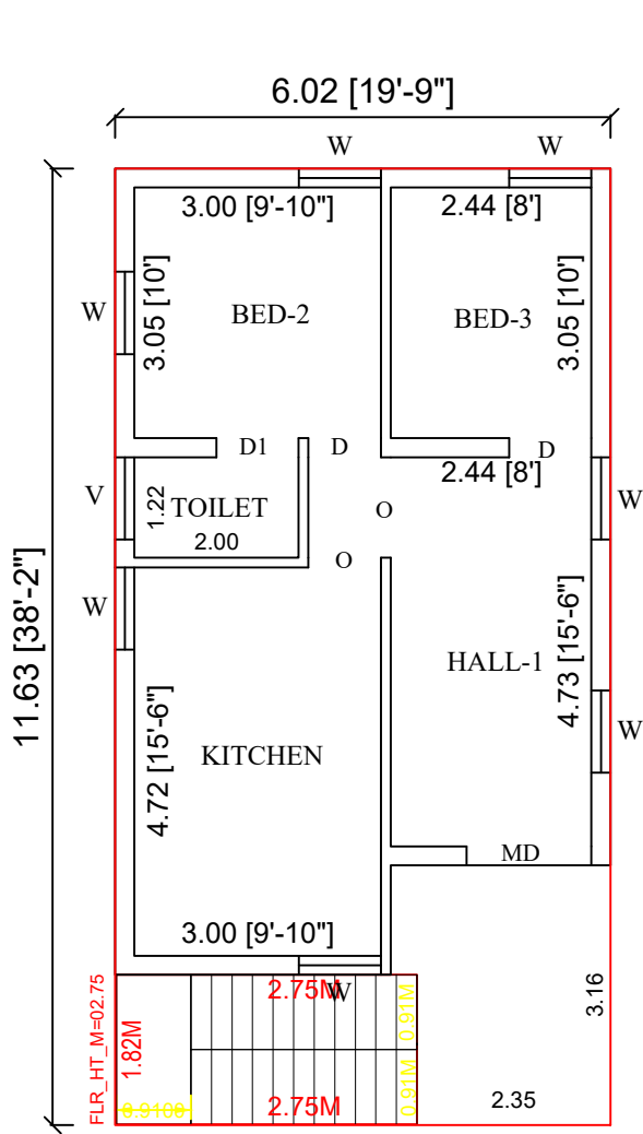
EX.GROUND FLOOR PLAN
