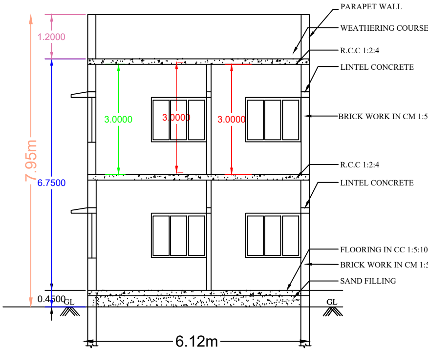
SECTION AB
