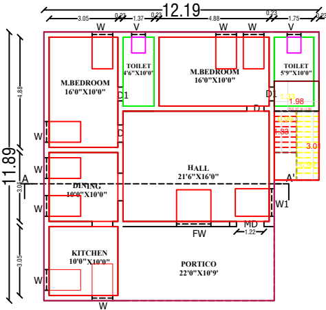
GROUND FLOOR PLAN FACING EAST
