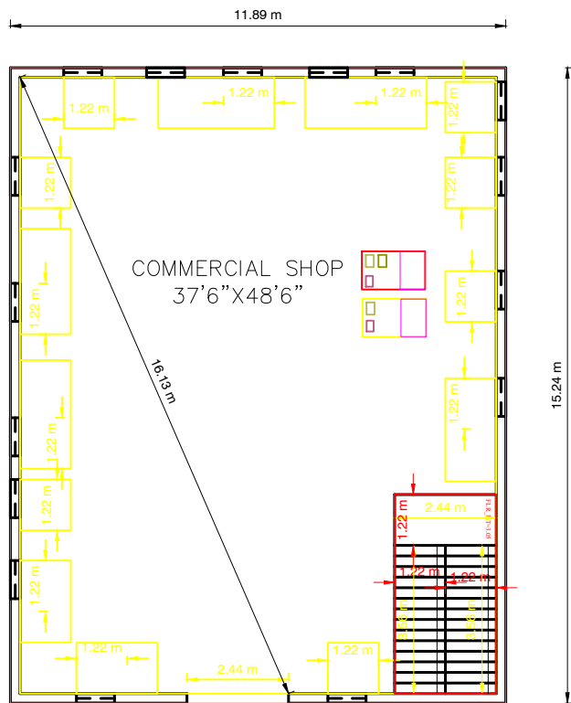
GROUND FLOOR PLAN [SOUTH FACING]
