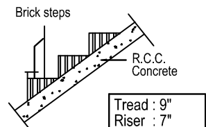
STAIRCASE DETAILS
