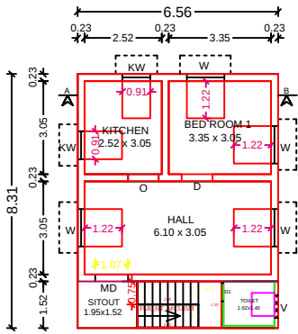
GROUND FLOOR PLAN (NORTH FACING)
