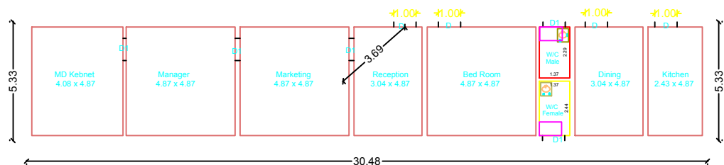
PRO.GROUND FLOOR PLAN
