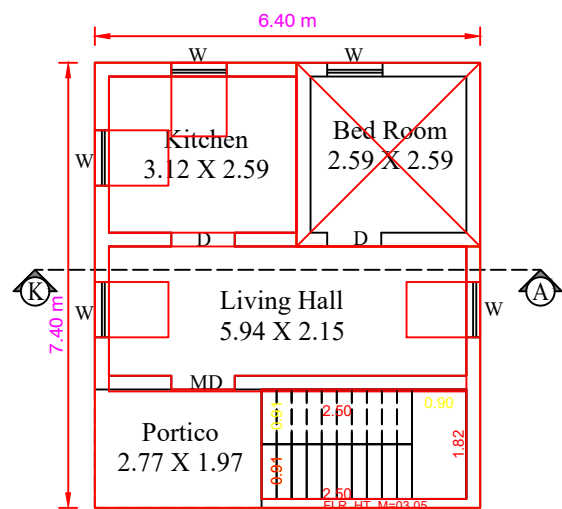
EXISTING & PROPOSED GROUND FLOOR PLAN
