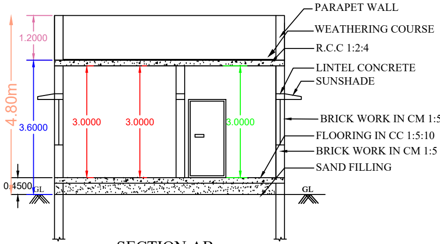
SECTION AB
