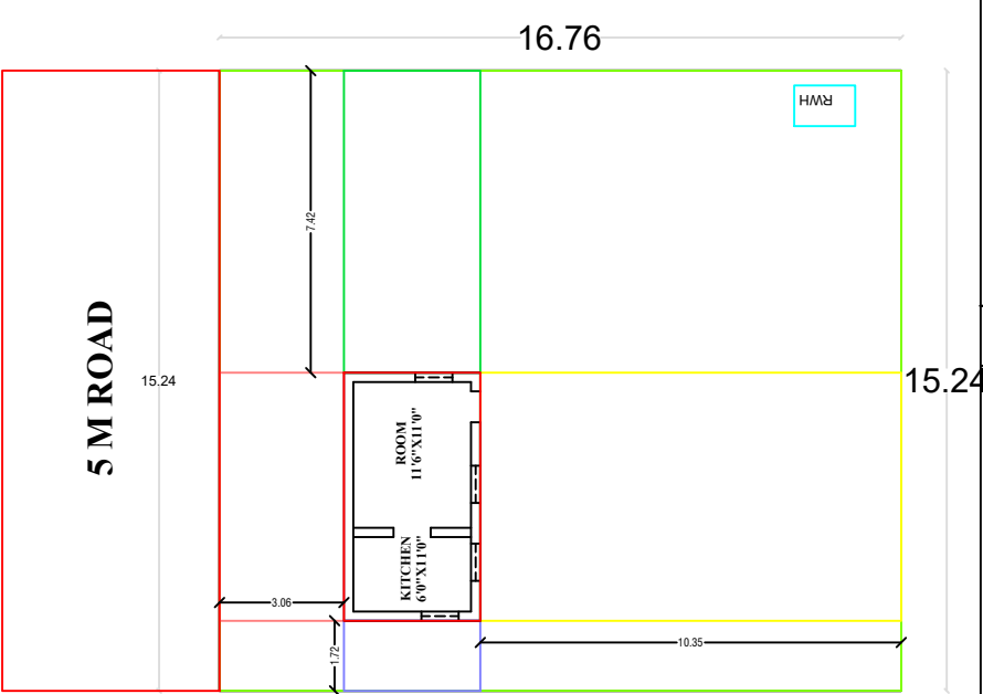
GROUND FLOOR PLAN FACING EAST
