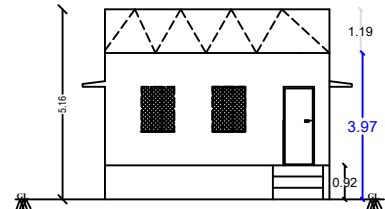
ELEVATION FACING EAST
