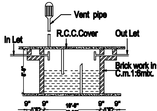
SEPTIC TANK DETAILS (NOT TO SCALE)
