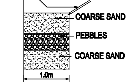
RAIN WATER PERCOLATION BED (NOT TO SCALE)
