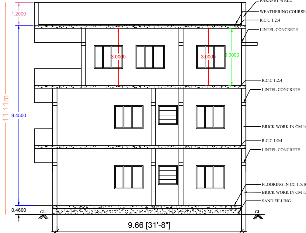
SECTION AB
