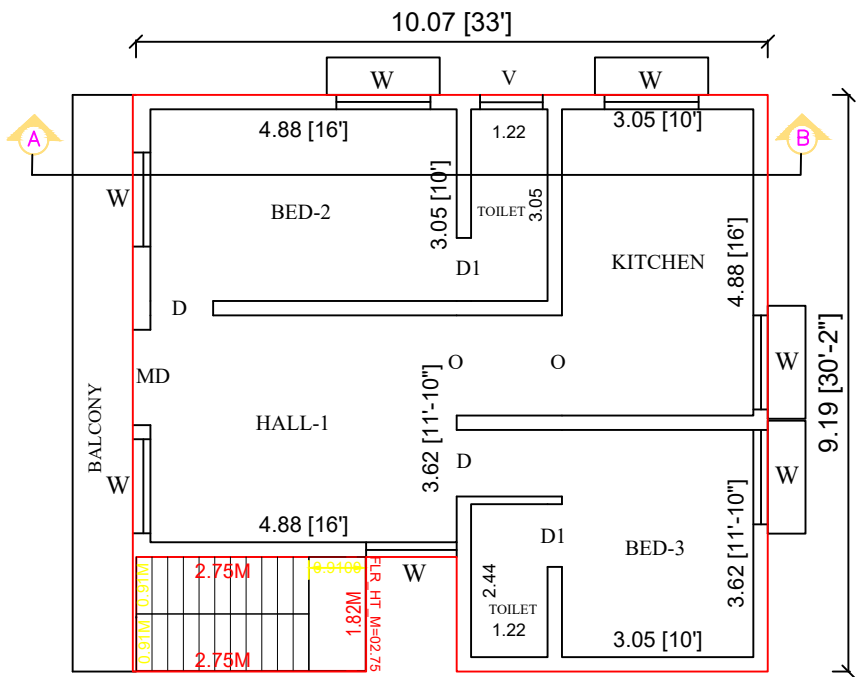
EXG.FIRST FLOOR PLAN
