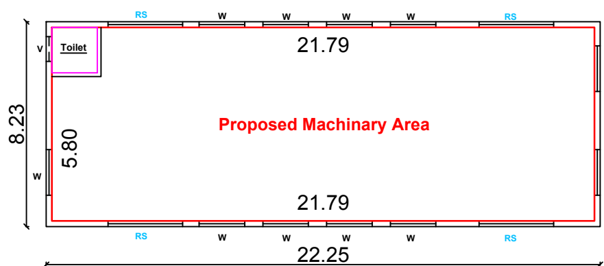
PROPOSED GROUND FLOOR PLAN
