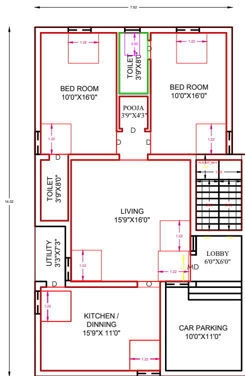
GROUND FLOOR PLAN [EAST FACING]
