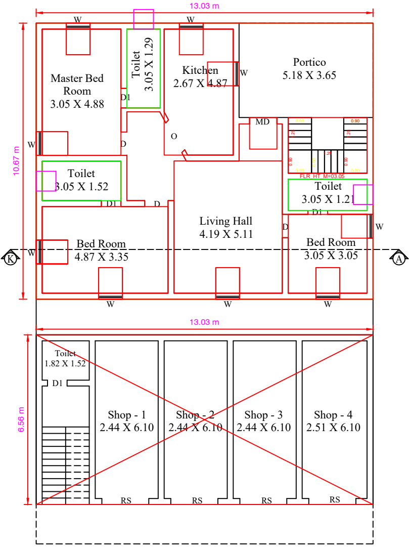
EXISTING & ADDITIONAL GROUND FLOOR PLAN
