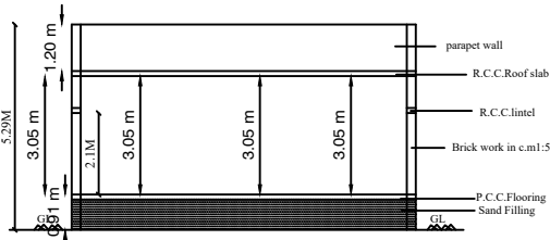
SECTION-"SR"
