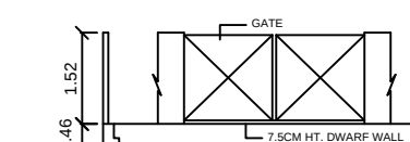
COMPOUND WALL WITH DWARF WALL DETAILS
