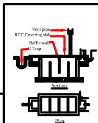
Section - 'CD'
