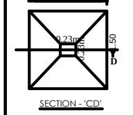
Foundation Detail - A
