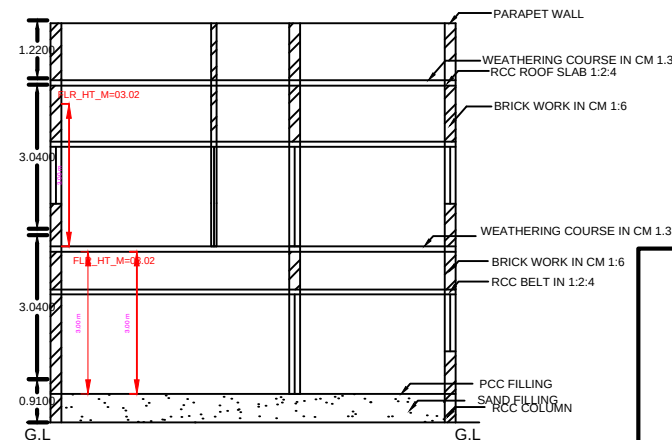
SECTION ON-AA&BB
