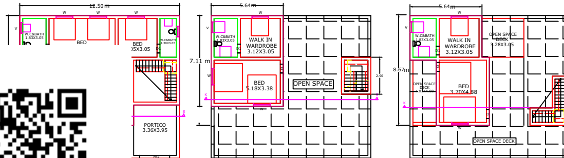
PLAN
