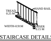
STAIRCASE DETAILS
