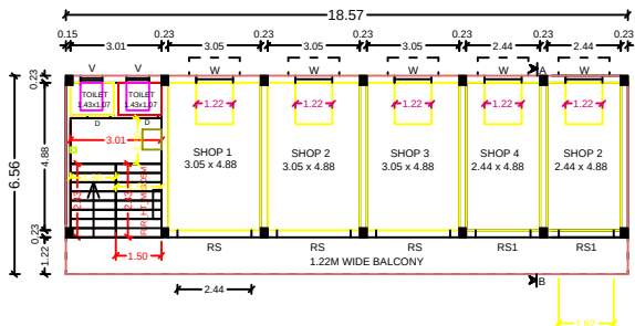
GROUND FLOOR PLAN (WEST FACING)
