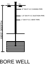
BORE WELL
